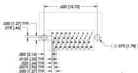
SIZE 37 - VIEW A
