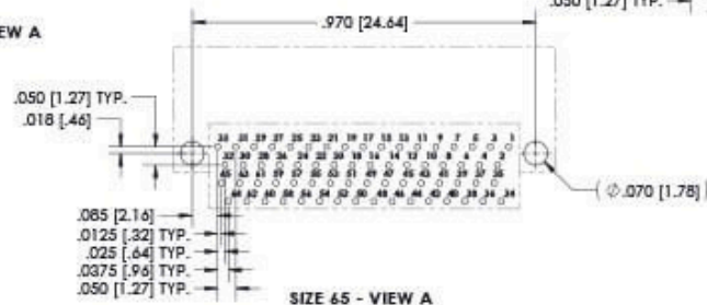
SIZE 65 - VIEW A
