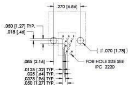
SIZE 9 - VIEW A
