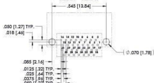
SIZE 31 - VIEW A
