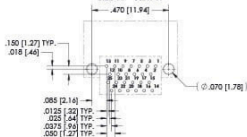
SIZE 25 - VIEW A
